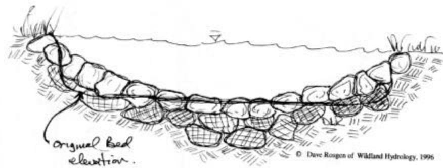
Cross-section View of Cross Vane Weir Design
